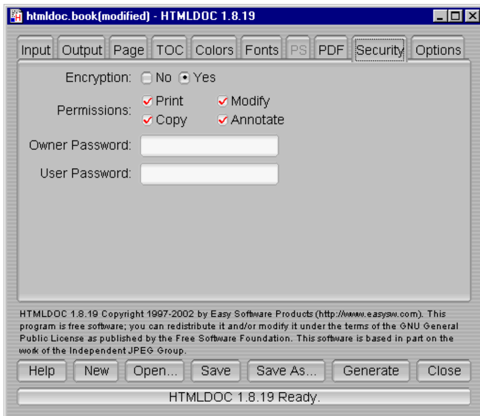
Figure 7-9 – The Security Tab
